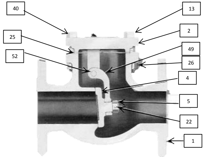
TYPICAL CRYOGENIC SWING CHECK VALVE
