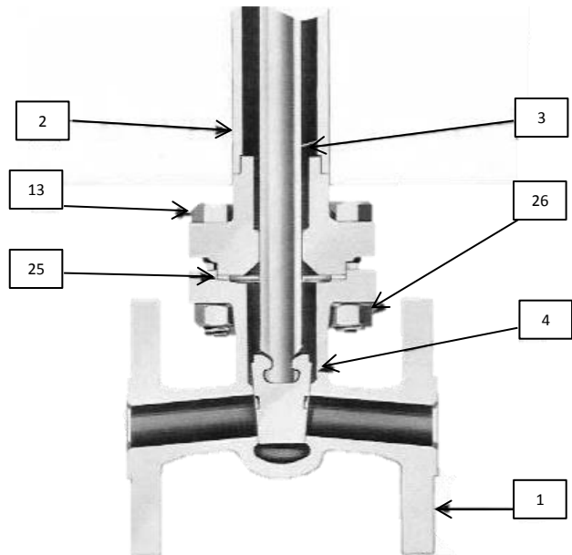
TYPICAL CRYOGENIC GATE VALVE
